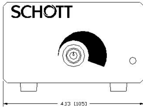
iQ121 LED Controller A25275
