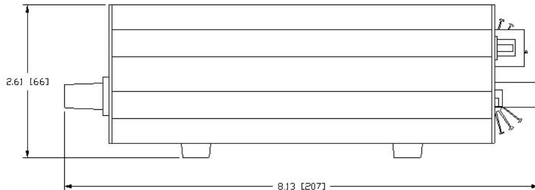
iQ121 LED Controller A25275
